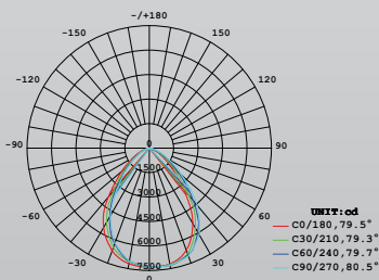
100W- Intensity Distribution Diagram in C Plans
