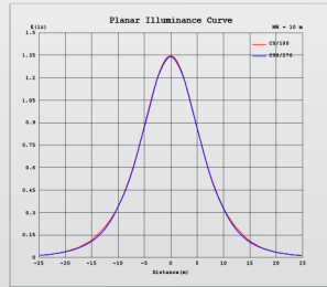
30W Planar Illuminance Curve
