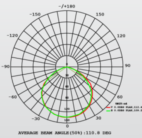
30W- Luminous Intensity Distribution
