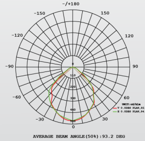
60W- Luminous Intensity Distribution
