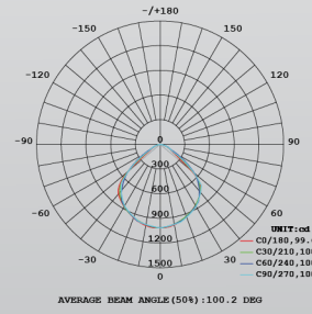
150W- Luminous Intensity Distribution
