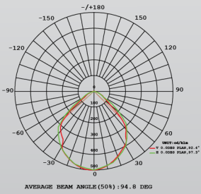
100W- Luminous Intensity Distribution
