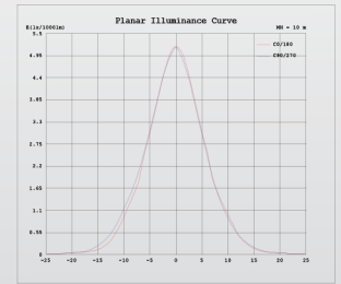
60W Planar Illuminance Curve
