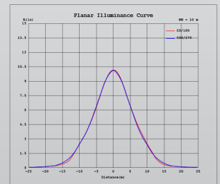
150W Planar Illuminance Curve
