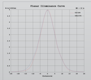
100W Planar Illuminance Curve
